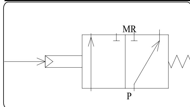
FUNCTIONAL DIAGRAM
