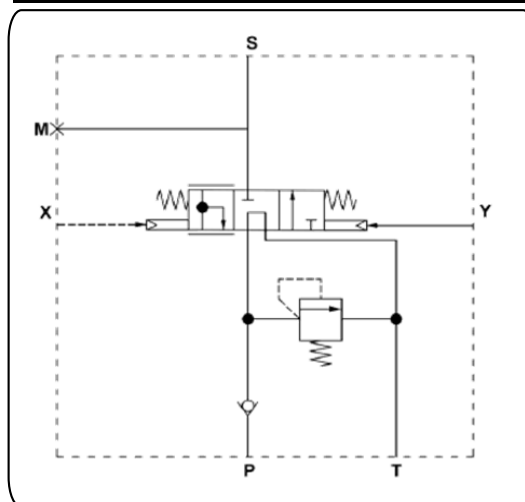
FUNCTIONAL DIAGRAM
