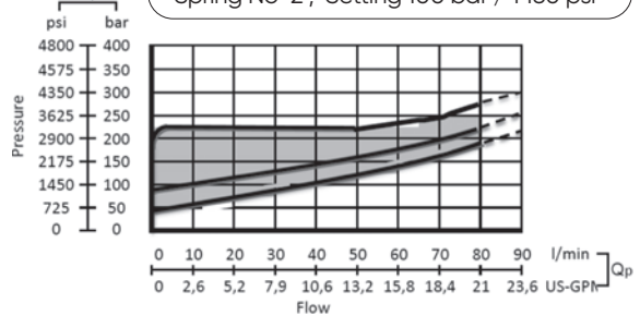
Spring No=2, Setting 100 bar / 1450 psi
